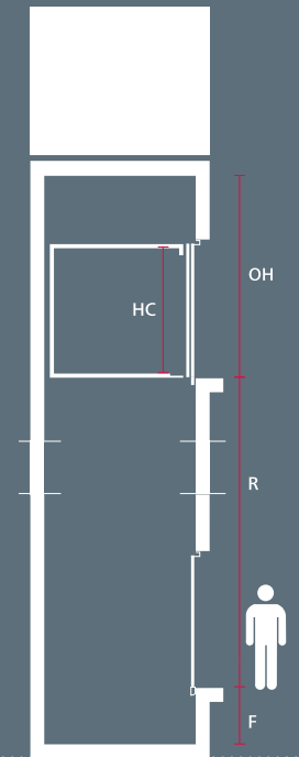
STANDARD ENTRANCE
